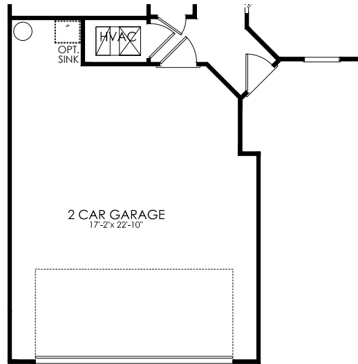
4' Garage Extension
